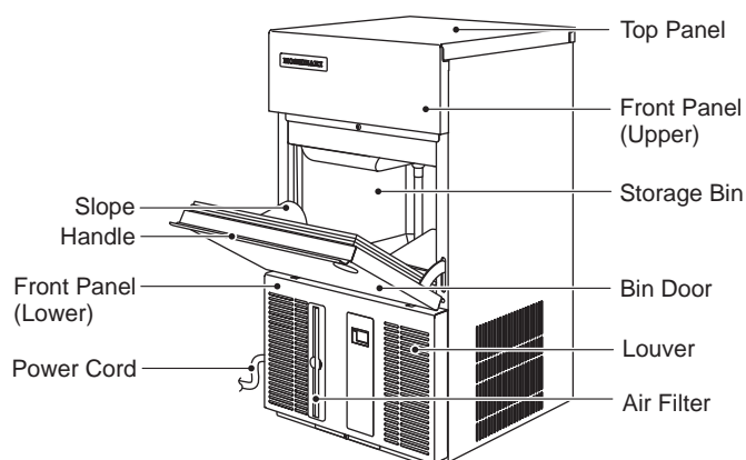
[IM-21CNE-HC, 30CNE/CWNE-HC]
