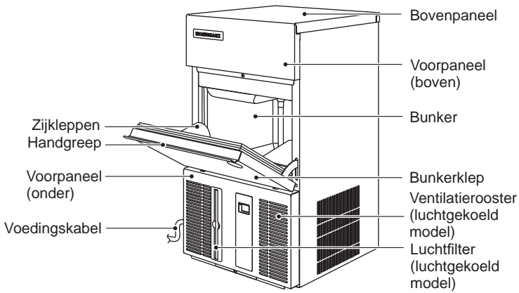
[IM-21CNE-HC, 30CNE/CWNE-HC]
